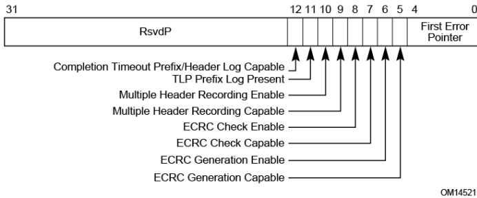
Figure 7-39: Advanced Error Capabilities and Control Register
