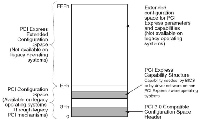
Figure 7-3: PCI Express Configuration Space Layout
