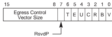
Figure 7-77: ACS Capability Register
