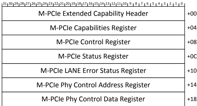
Figure 7-138. M-PCIe Extended Capability
