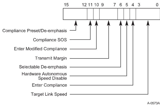
Figure 7-28: Link Control 2 Register
