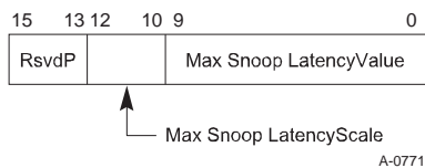
Figure 7-125: Max Snoop Latency Register
