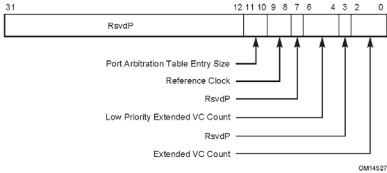
Figure 7-47: Port VC Capability Register 1
