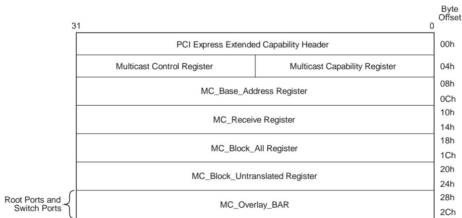
Figure 7-99: Multicast Extended Capability Structure
