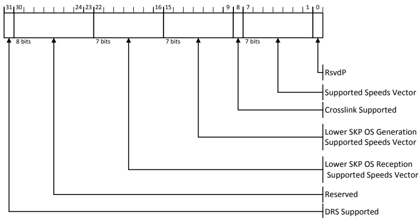
Figure 7-27: Link Capabilities 2 Register
