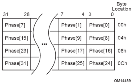
Figure 7-54: Example VC Arbitration Table with 32 Phases
