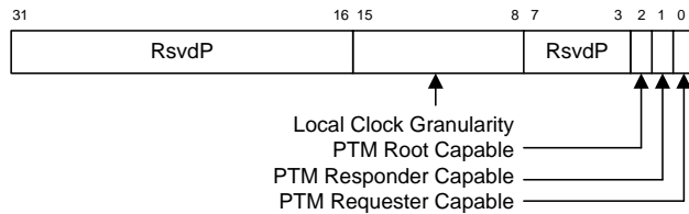
Figure 7-166: PTM Capability Register
