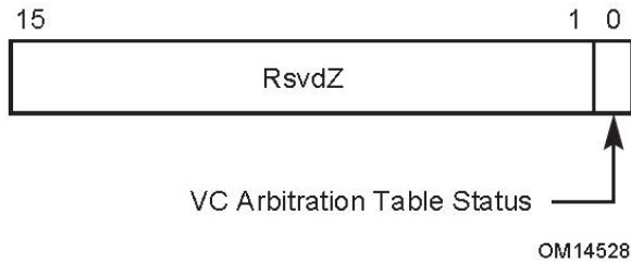
Figure 7-87: Port VC Status Register
