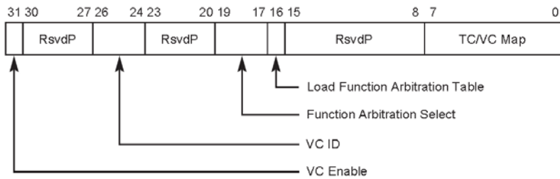
Figure 7-89: VC Resource Control Register
