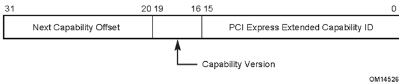
Figure 7-92: Vendor-Specific Extended Capability Header
