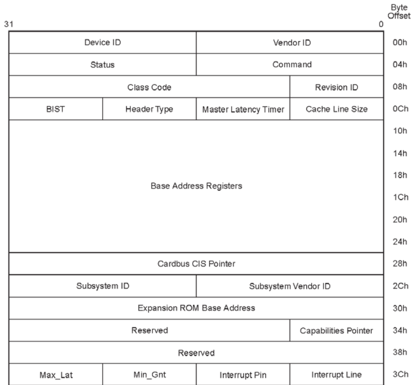
Figure 7-5: Type 0 Configuration Space Header
