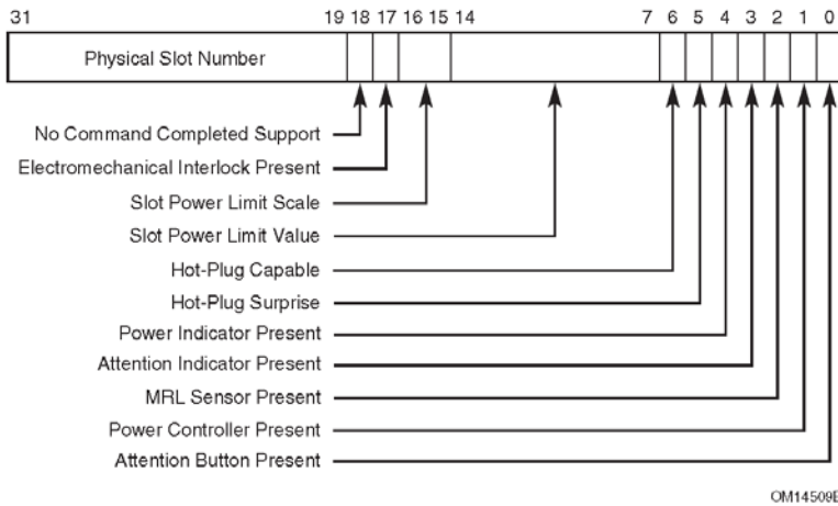
Figure 7-19: Slot Capabilities Register
