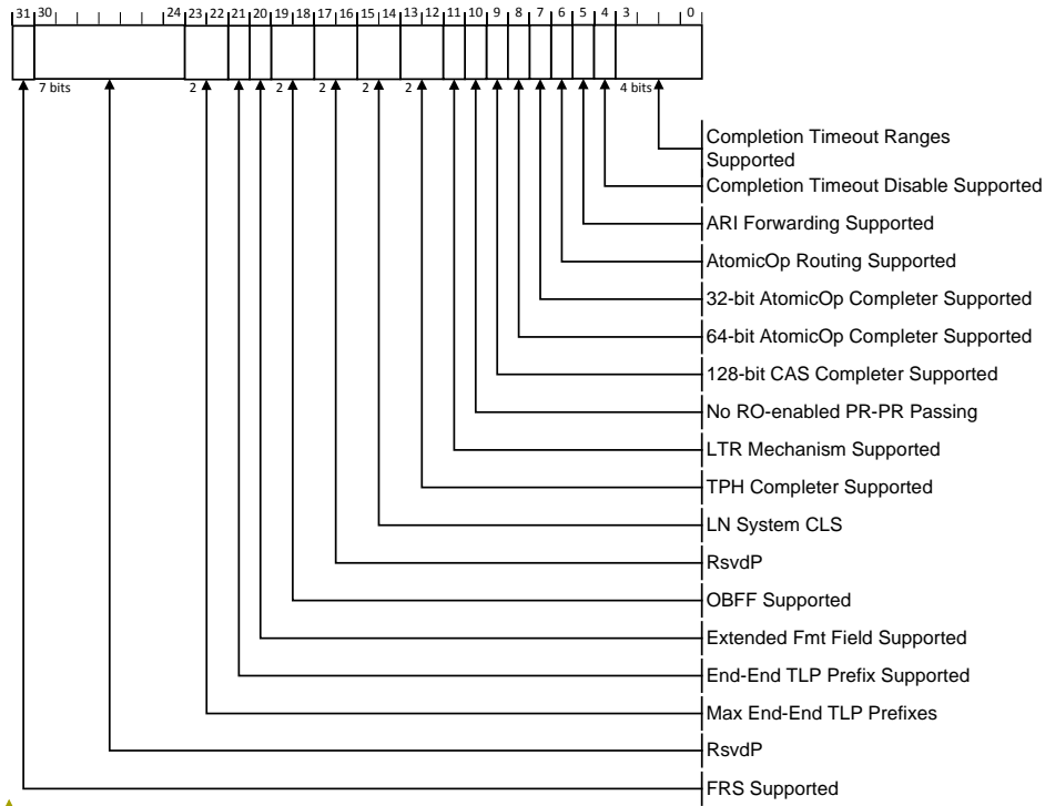
Figure 7-25: Device Capabilities 2 Register
