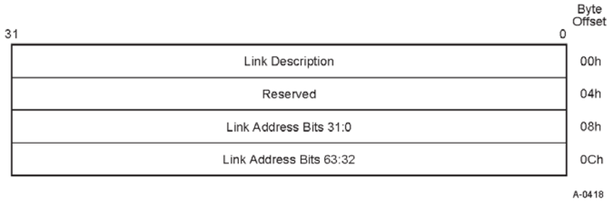
Figure 7-64: Link Address for Link Type 0
