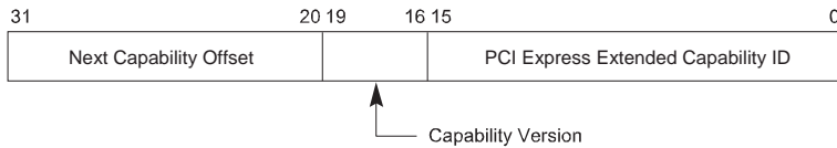
Figure 7-109: Resizable BAR Extended Capability Header
