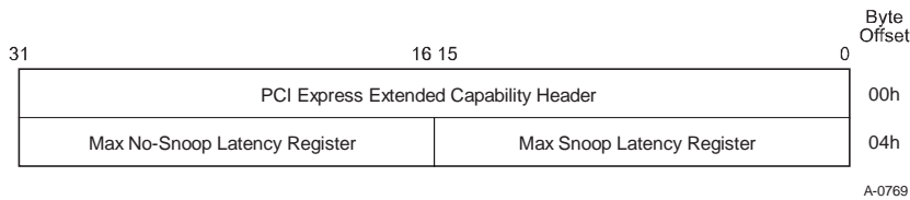
Figure 7-123: LTR Extended Capability Structure
