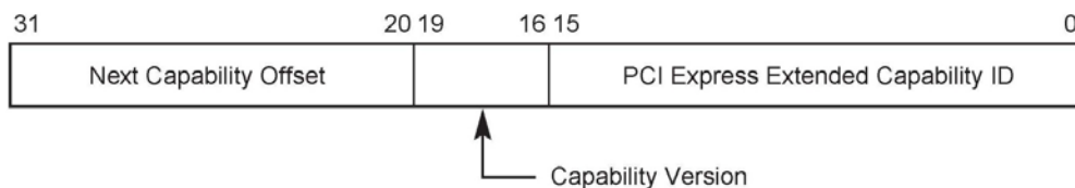
Figure 7-60: Root Complex Link Declaration Extended Capability Header
