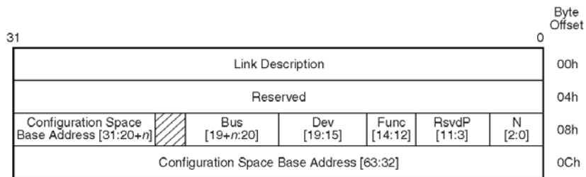
Figure 7-65: Link Address for Link Type 1
