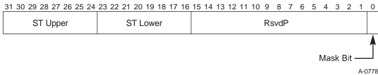
Figure 7-9: Vector Control for MSI-X Table Entries
