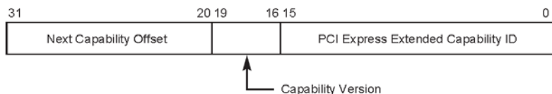
Figure 7-33: Advanced Error Reporting Extended Capability Header
