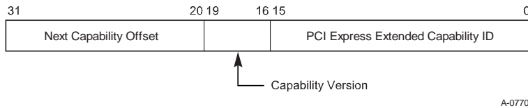
Figure 7-124: LTR Extended Capability Header
