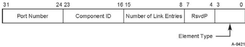
Figure 7-61: Element Self Description Register
