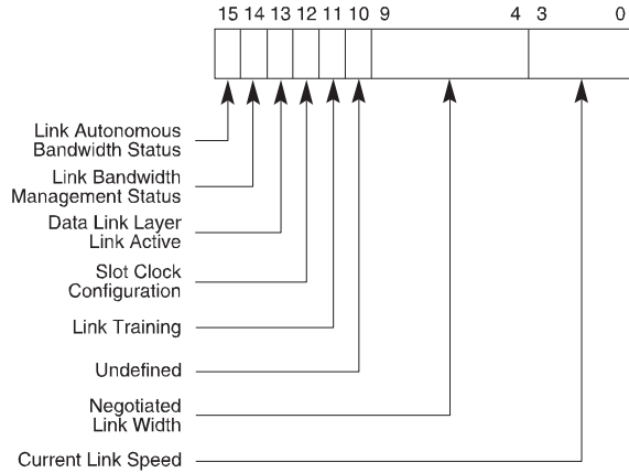
Figure 7-18: Link Status Register
