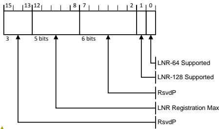
Figure 7-148: LNR Capability Register
