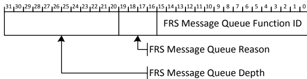
Figure 7-178: FRS Message Queue Register
