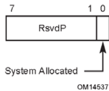
Figure 7-74: Power Budget Capability Register
