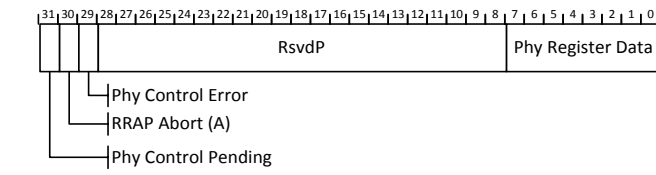
Figure 7-145: M-PCIe Phy Control Data Register
