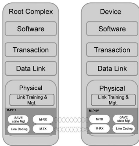
Figure 8-1: Adaptation of MIPI-M-PHY
