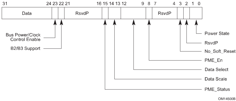
Figure 7-8: Power Management Status/Control Register
