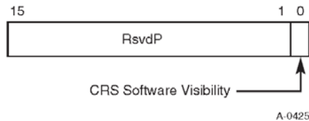
Figure 7-23: Root Capabilities Register
