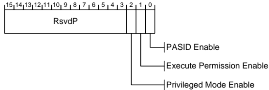
Figure 7-141: PASID Control Register
