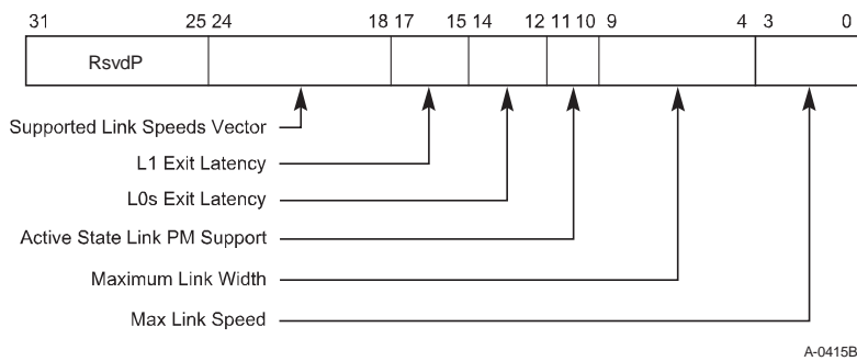
Figure 7-68: Root Complex Link Capabilities Register
