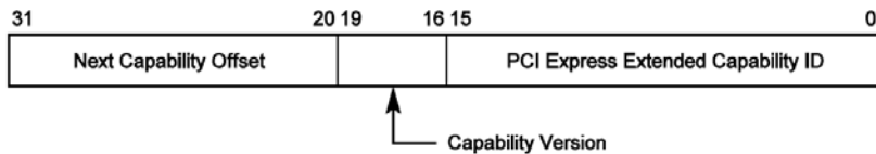
Figure 7-139. M-PCIe Extended Capability Header
