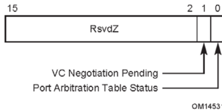
Figure 7-53: VC Resource Status Register
