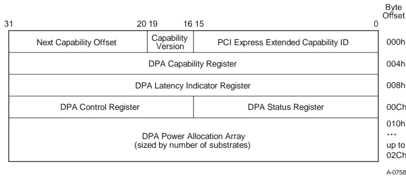
Figure 7-116: Dynamic Power Allocation Capability Structure
