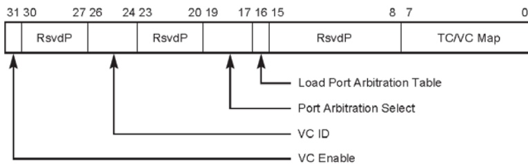
Figure 7-52: VC Resource Control Register
