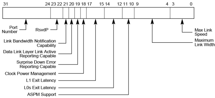
Figure 7-16: Link Capabilities Register
