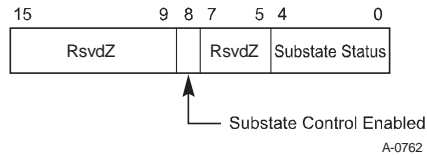
Figure 7-120: DPA Status Register
