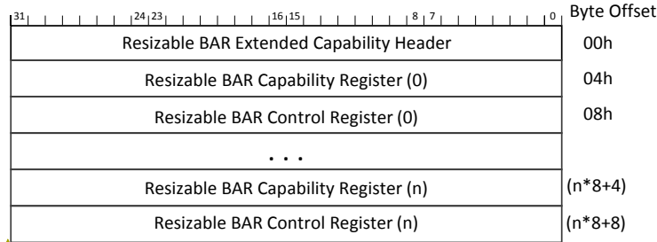
Figure 7-108: Resizable BAR Capability
