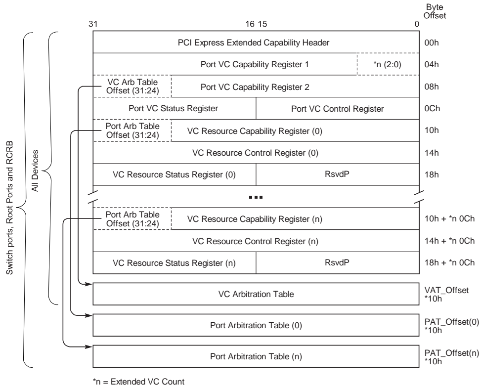
Figure 7-45: PCI Express Virtual Channel Capability Structure
