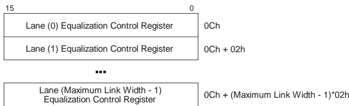
Figure 7-136: Lane Equalization Control Register
