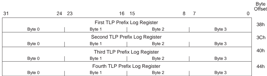
Figure 7-44: TLP Prefix Log Register
