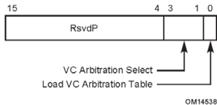
Figure 7-49: Port VC Control Register
