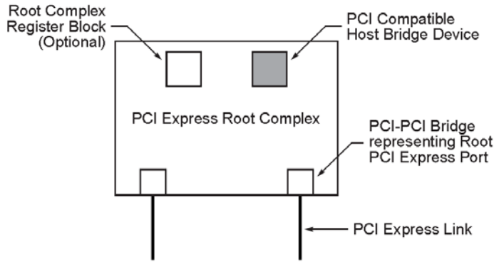
Figure 7-1: PCI Express Root Complex Device Mapping
