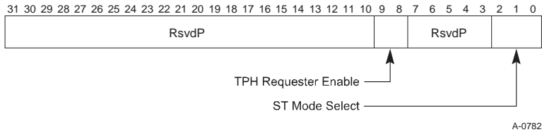
Figure 7-130: TPH Requester Control Register
