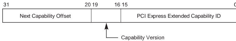
Figure 7-117: DPA Extended Capability Header
