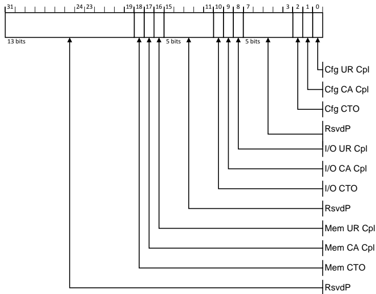
Figure 7-157: RP PIO Mask Register
