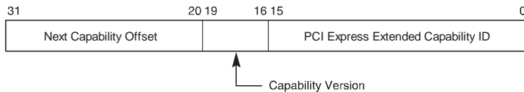
Figure 7-76: ACS Extended Capability Header
