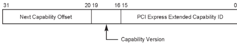
Figure 7-95: RCRB Header Extended Capability Header
