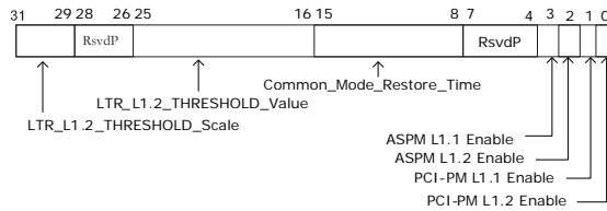
Figure 7-171: L1 PM Substates Control 1 Register
