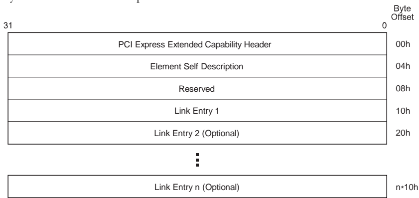
Figure 7-59: PCI Express Root Complex Link Declaration Capability
