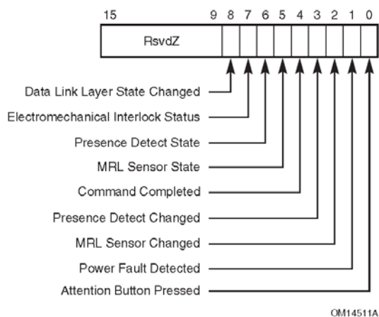
Figure 7-21: Slot Status Register
