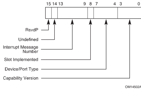
Figure 7-12: PCI Express Capabilities Register
