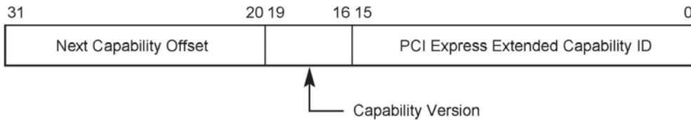
Figure 7-169: L1 PM Substates Extended Capability Header
