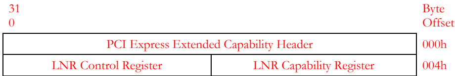
Figure 7-146: LNR Extended Capability
