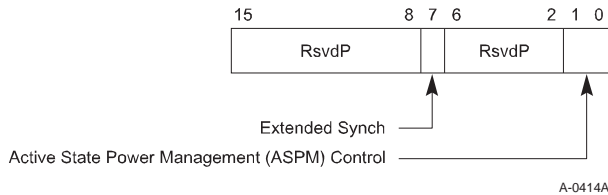
Figure 7-69: Root Complex Link Control Register
