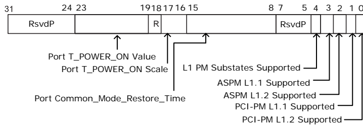
Figure 7-170: L1 PM Substates Capabilities Register
