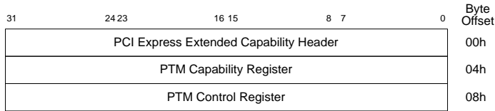
Figure 7-164: PTM Extended Capability Structure
