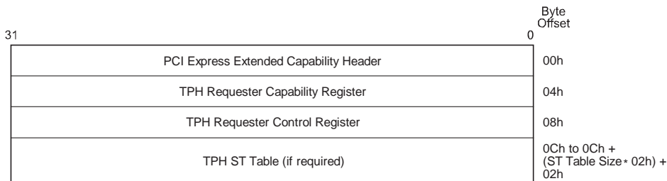
Figure 7-127: TPH Extended Capability Structure
