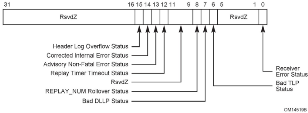
Figure 7-37: Correctable Error Status Register
