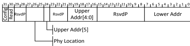
Figure 7-144: M-PCIe Phy Control Address Register
