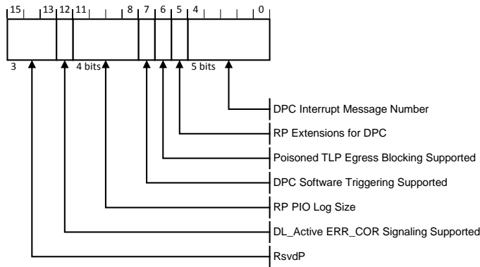
Figure 7-152: DPC Capability Register
