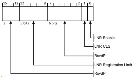
Figure 7-149: LNR Control Register
