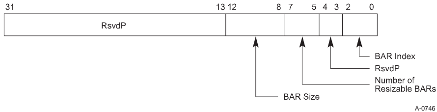
Figure 7-111: Resizable BAR Control Register
