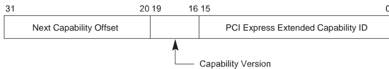
Figure 7-100: Multicast Extended Capability Header
