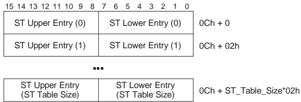
Figure 7-131: TPH ST Table
