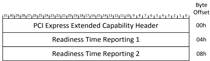
Figure 7-179: Readiness Time Reporting Extended Capability
