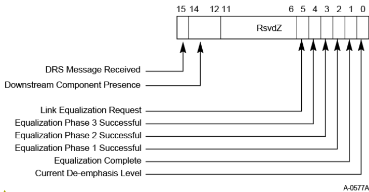
Figure 7-29: Link Status 2 Register
