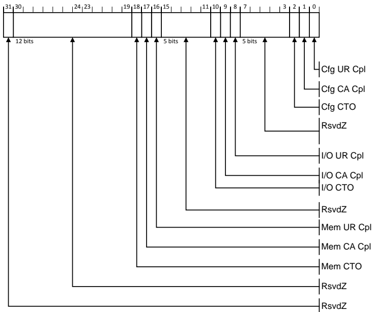
Figure 7-156: RP PIO Status Register
