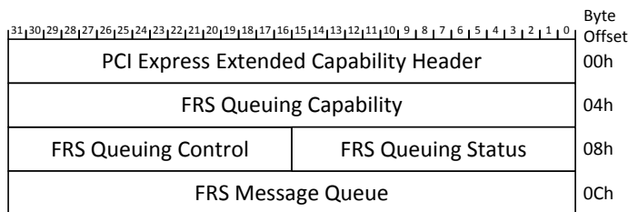
Figure 7-173: FRS Extended Capability
