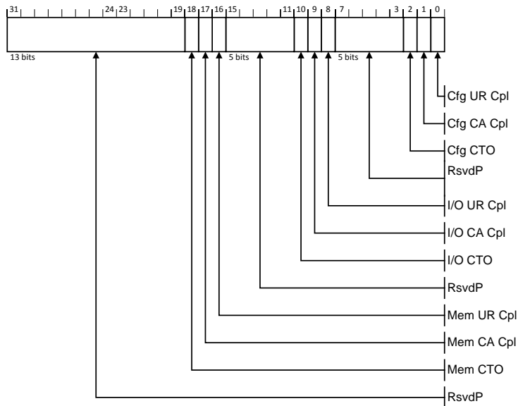
Figure 7-159: RP PIO SysError Register
