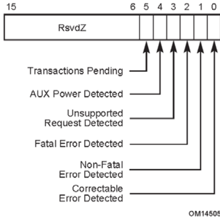
Figure 7-15: Device Status Register
