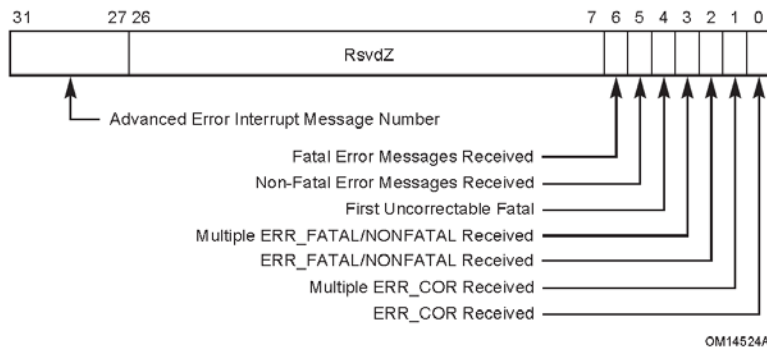
Figure 7-42: Root Error Status Register
