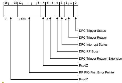
Figure 7-154. DPC Status Register
