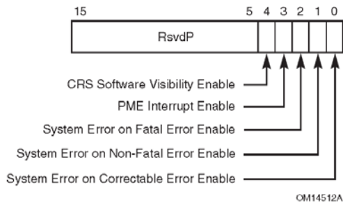
Figure 7-22: Root Control Register
