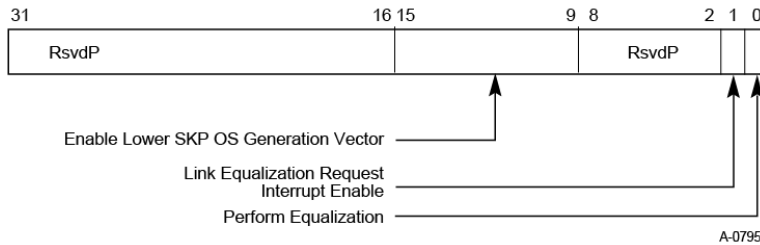
Figure 7-134: Link Control 3 Register
