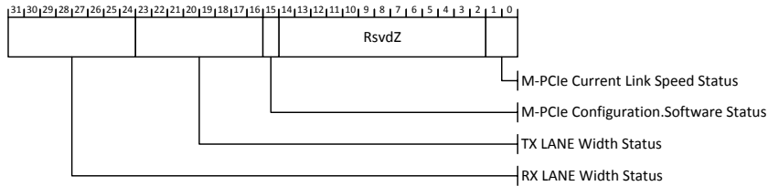
Figure 7-142: M-PCIe Status Register
