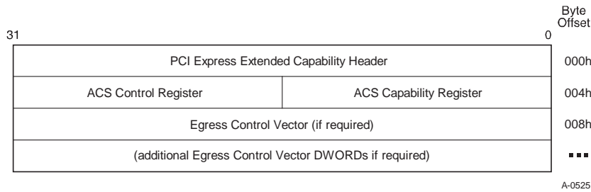
Figure 7-75: ACS Extended Capability
