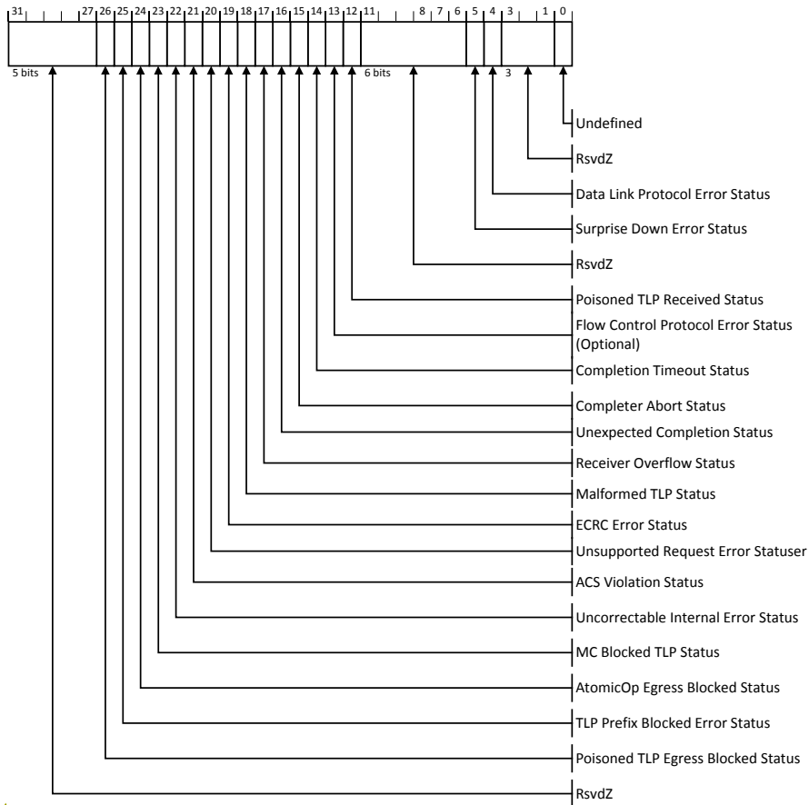
Figure 7-34: Uncorrectable Error Status Register
