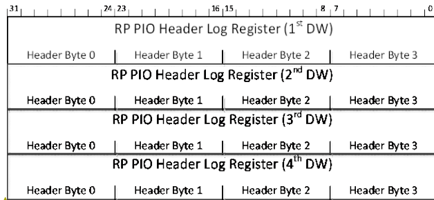
Figure 7-161: RP PIO Header Log Register
