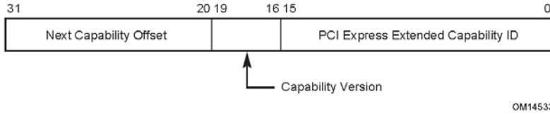
Figure 7-57: Device Serial Number Extended Capability Header
