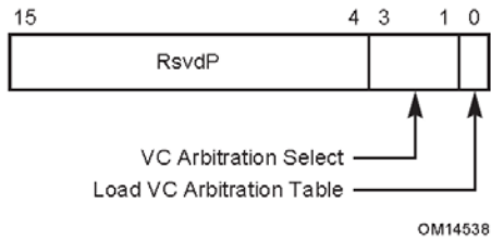
Figure 7-86: Port VC Control Register
