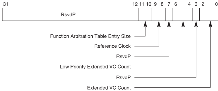
Figure 7-84: Port VC Capability Register 1
