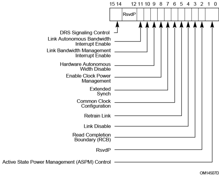
Figure 7-17: Link Control Register
