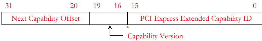
Figure 7-147: LNR Extended Capability Header
