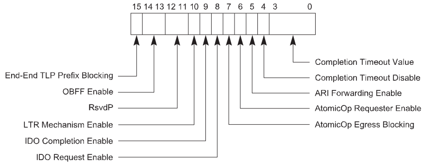
Figure 7-26: Device Control 2 Register
