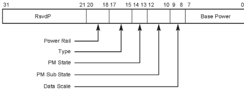
Figure 7-73: Power Budgeting Data Register
