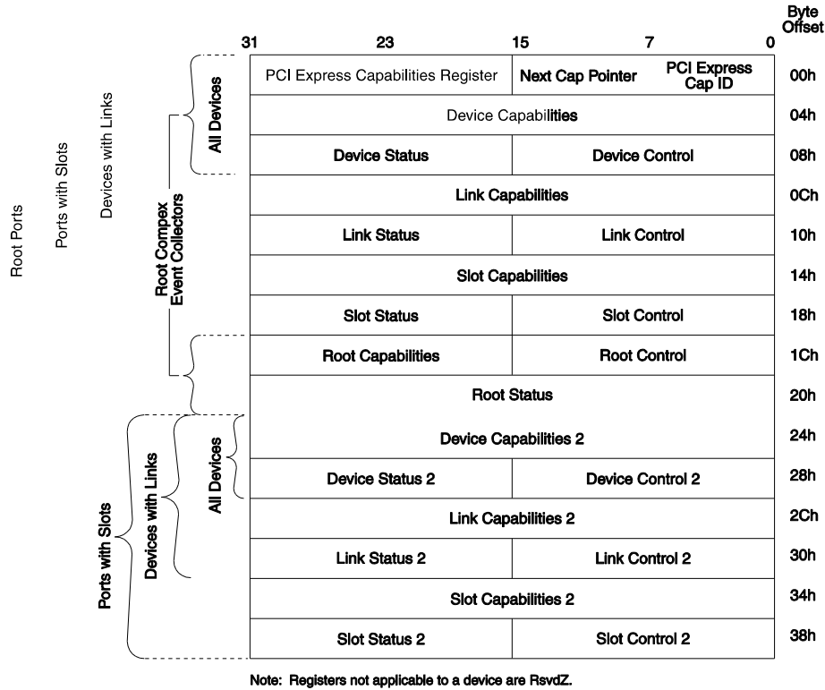
Figure 7-10: PCI Express Capability Structure
