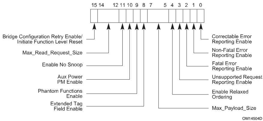
Figure 7-14: Device Control Register
