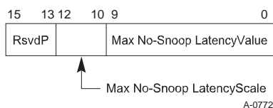
Figure 7-126: Max No-Snoop Latency Register
