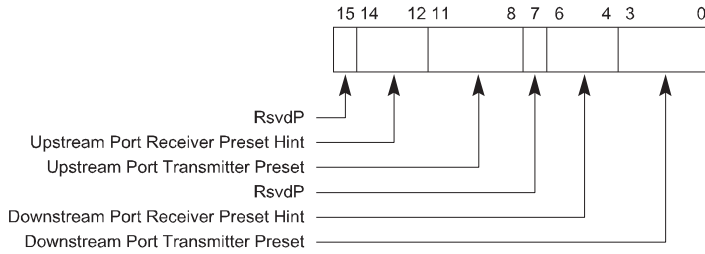
Figure 7-137: Lane ((Maximum Link Width - 1):0) Equalization Control Register
