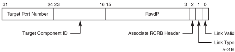
Figure 7-63: Link Description Register
