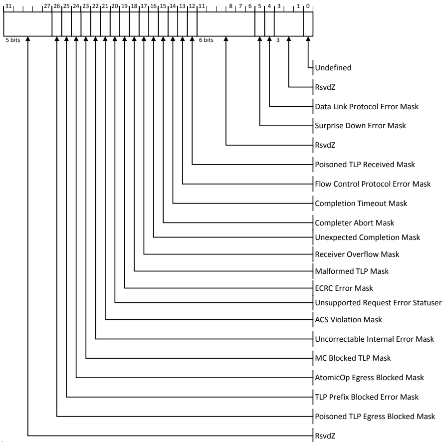
Figure 7-35: Uncorrectable Error Mask Register
