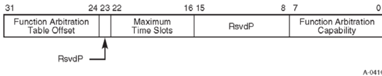
Figure 7-88: VC Resource Capability Register
