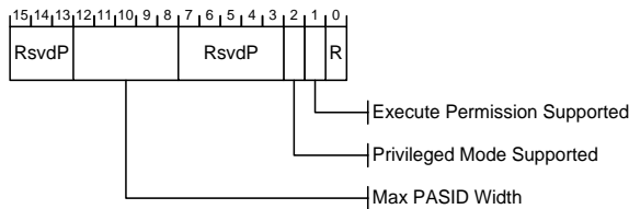
Figure 7-140: PASID Capability Register
