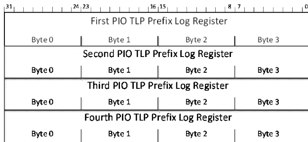
Figure 7-163: RP PIO TLP Prefix Log Register
