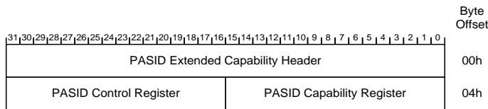
Figure 7-138: PASID Extended Capability Structure
