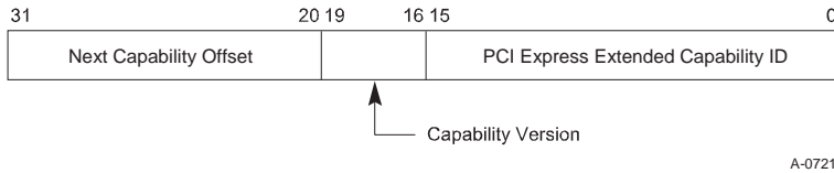
Figure 7-113: ARI Capability Header
