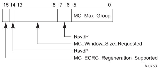
Figure 7-101: Multicast Capability Register
