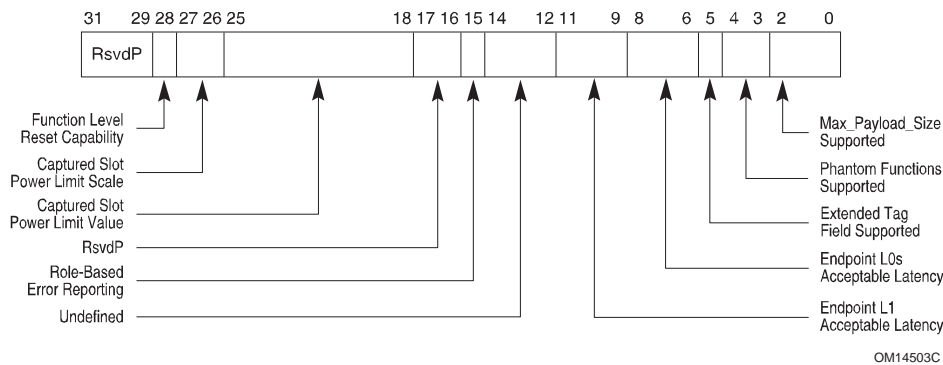
Figure 7-13: Device Capabilities Register
