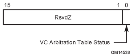
Figure 7-50: Port VC Status Register
