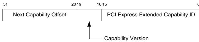
Figure 7-165: PTM Extended Capability Header
