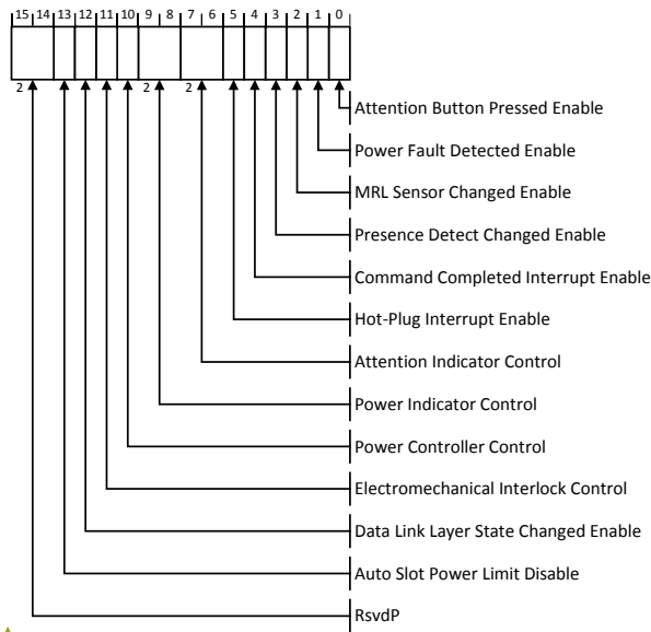
Figure 7-20: Slot Control Register
