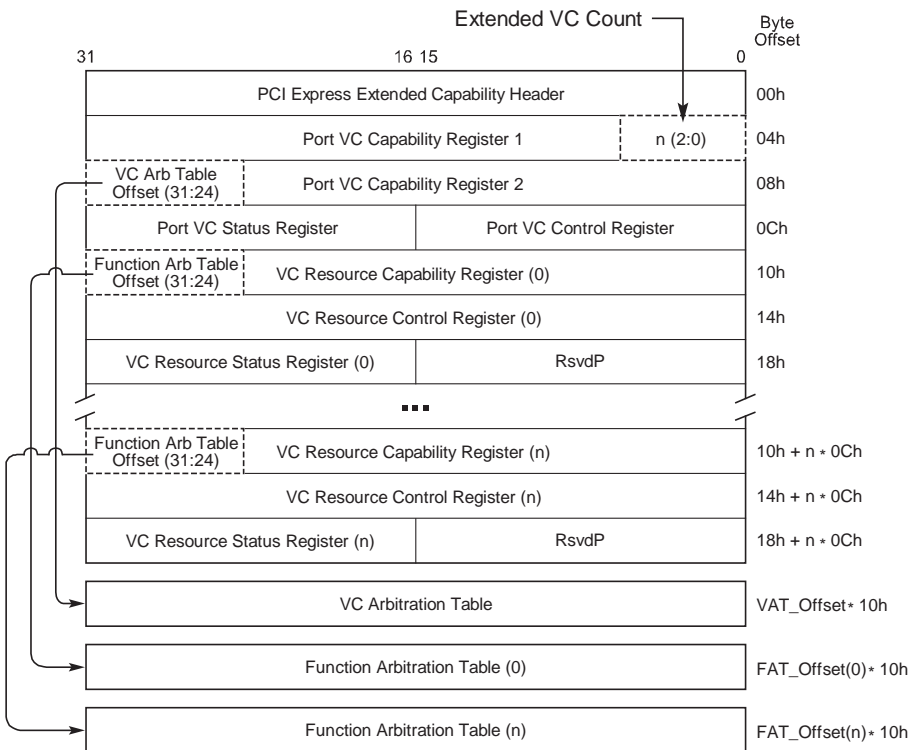
Figure 7-82: PCI Express MFVC Capability Structure
