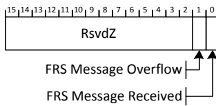
Figure 7-176: FRS Queuing Status Register
