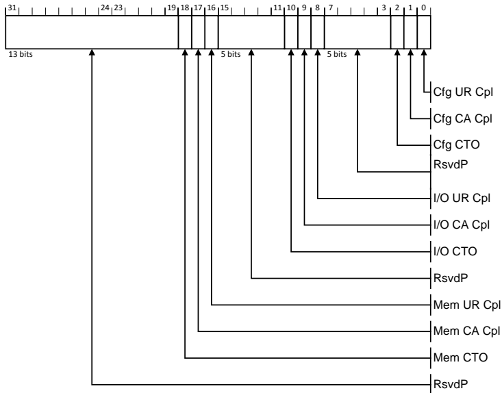
Figure 7-158: RP PIO Severity Register
