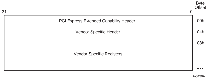
Figure 7-91: PCI Express VSEC Structure
