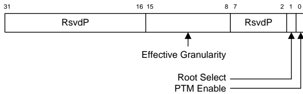
Figure 7-167: PTM Control Register
