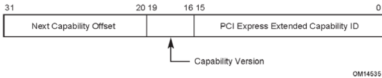
Figure 7-72: Power Budgeting Extended Capability Header
