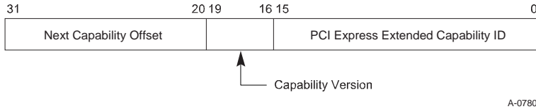
Figure 7-128: TPH Requester Extended Capability Header
