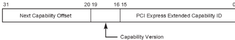
Figure 7-83: MFVC Extended Capability Header
