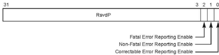
Figure 7-41: Root Error Command Register
