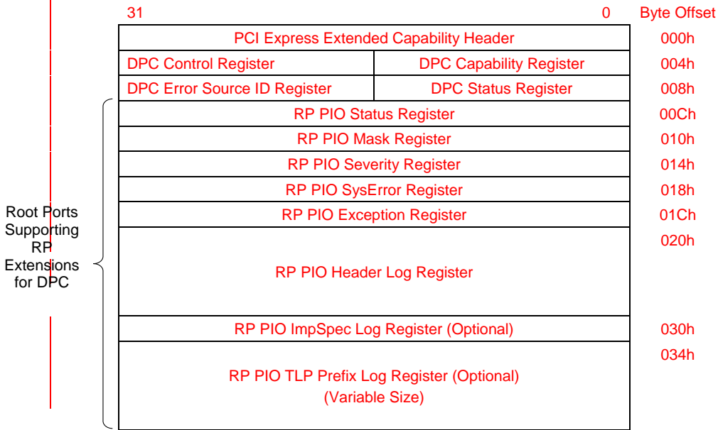
Figure 7-150: DPC Extended Capability
