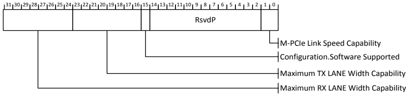
Figure 7-140: M-PCIe Capabilities Register
