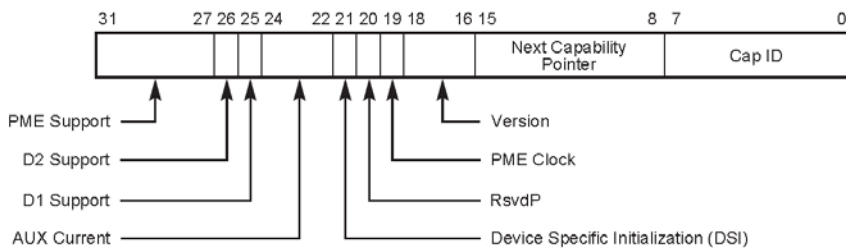
Figure 7-7: Power Management Capabilities Register
