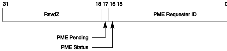
Figure 7-24: Root Status Register
