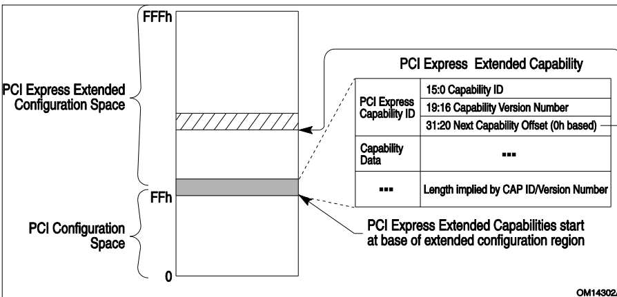
Figure 7-30: PCI Express Extended Configuration Space Layout
