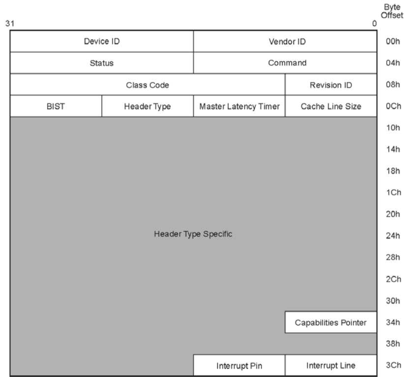
Figure 7-4: Common Configuration Space Header
