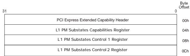
Figure 7-168: L1 PM Substates Capability
