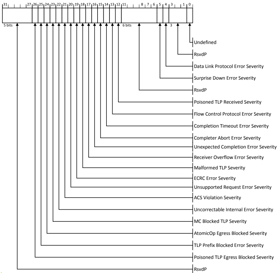
Figure 7-36: Uncorrectable Error Severity Register
