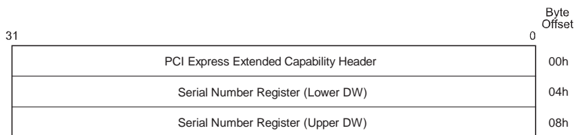
Figure 7-56: PCI Express Device Serial Number Capability Structure
