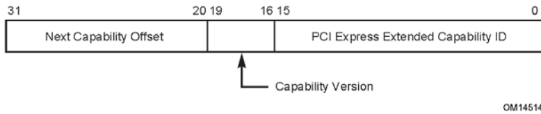
Figure 7-31: PCI Express Extended Capability Header
