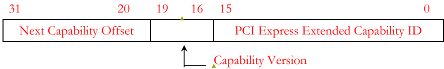
Figure 7-151: DPC Extended Capability Header
