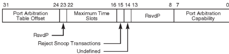
Figure 7-51: VC Resource Capability Register
