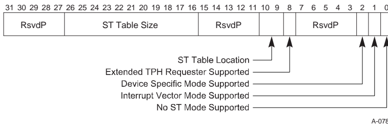
Figure 7-129: TPH Requester Capability Register
