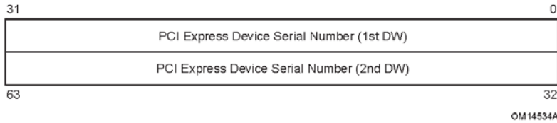
Figure 7-58: Serial Number Register
