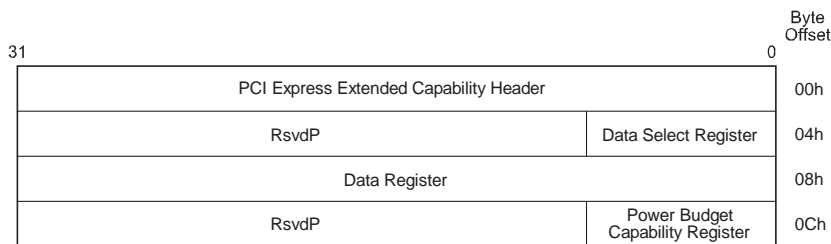
Figure 7-71: PCI Express Power Budgeting Capability Structure
