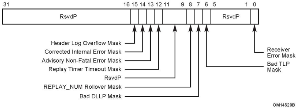
Figure 7-38: Correctable Error Mask Register
